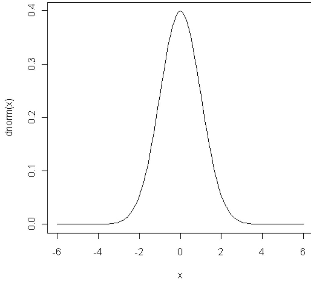
Standard normal
